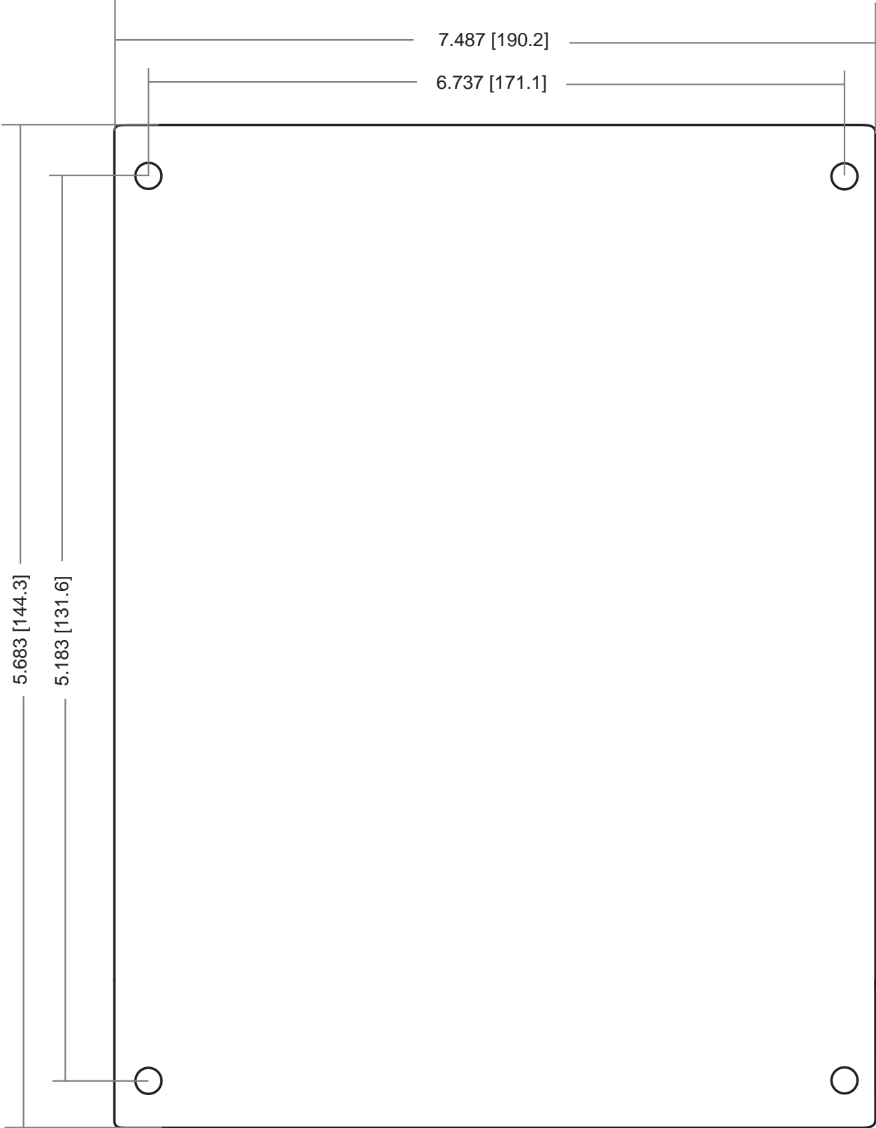
Figure 4.7.1 – Mounting Base Template with Hole Locations
